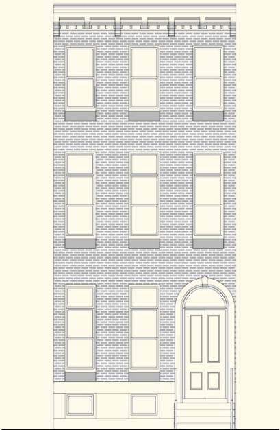
front elevation
