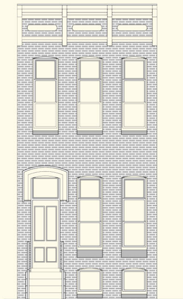
front elevation
