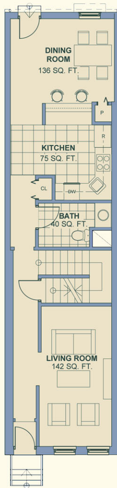
first floor
